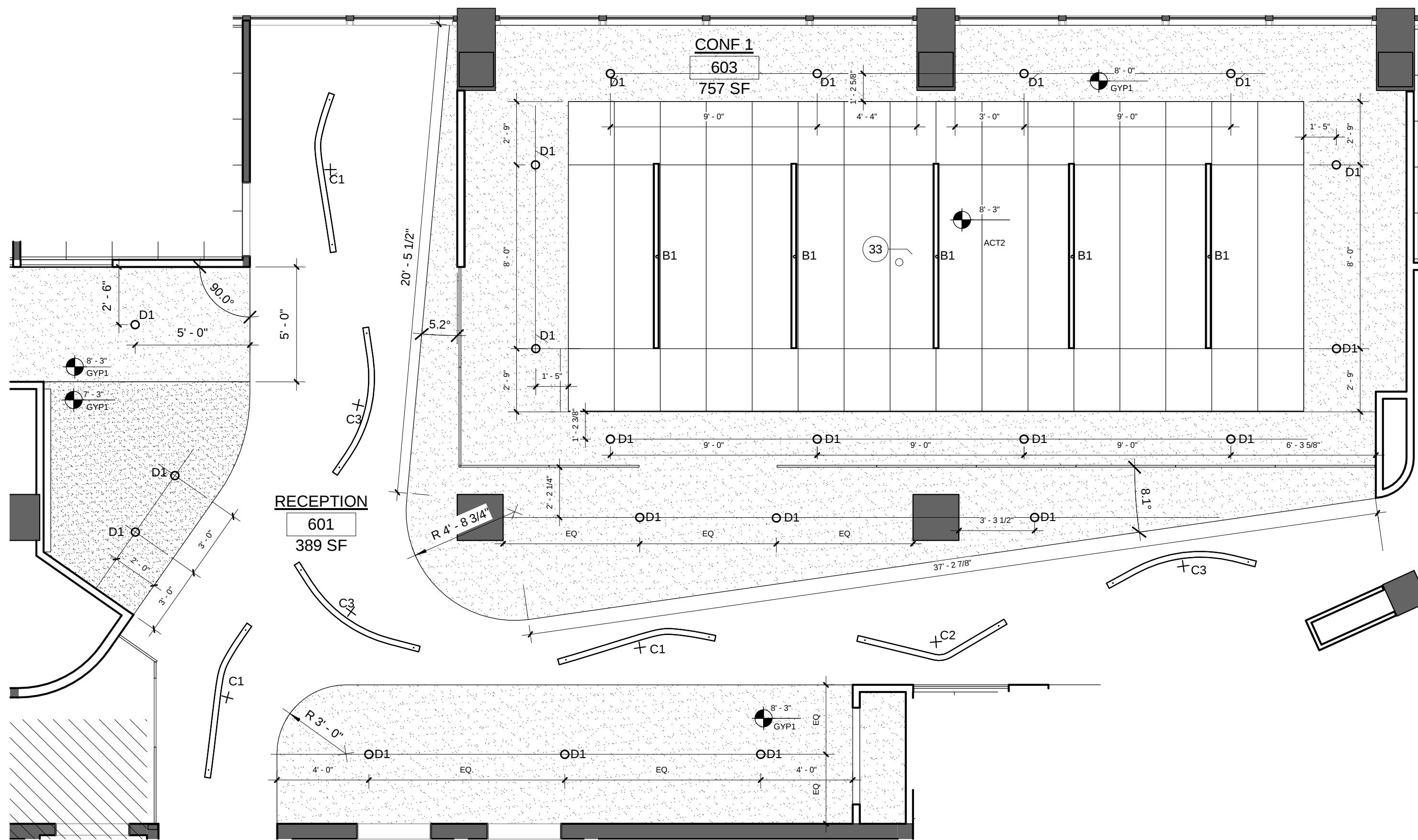
2 ENLARGED LOBBY CONFERENCE CEILING PLAN 1/4" = 1'-0"
