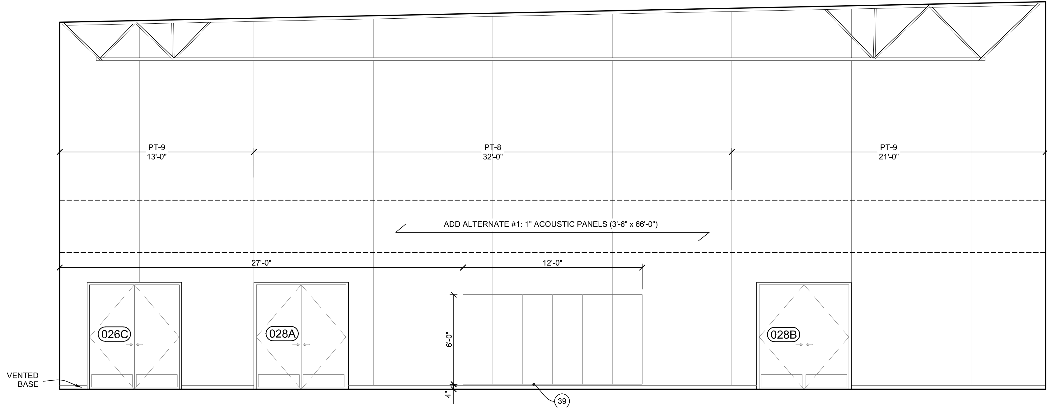
1 GYMNASIUM RM 026 A704 1/4" = 1'-0"
