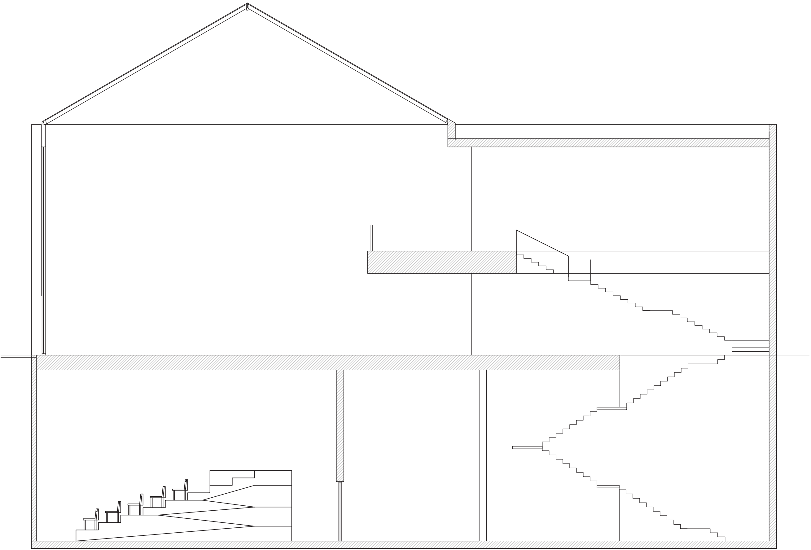
ATRIUM SECTION
